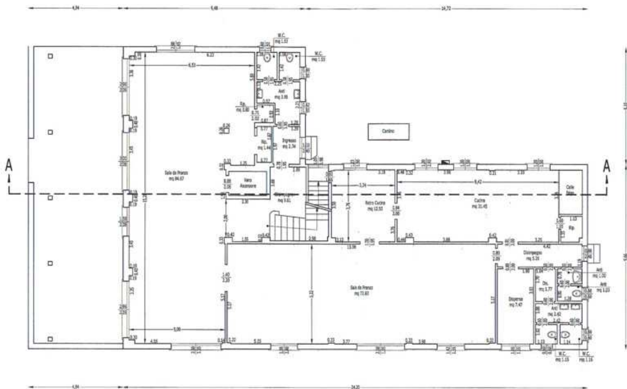
Piano Terra
